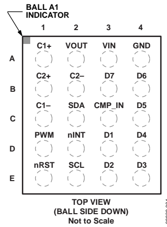
Figure 4. WLCSP Pin Configuration
