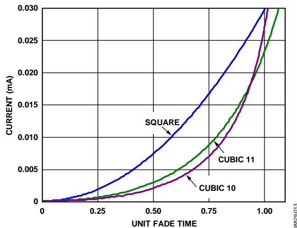
Figure 35. Comparison of the Dimming Transfers Laws
